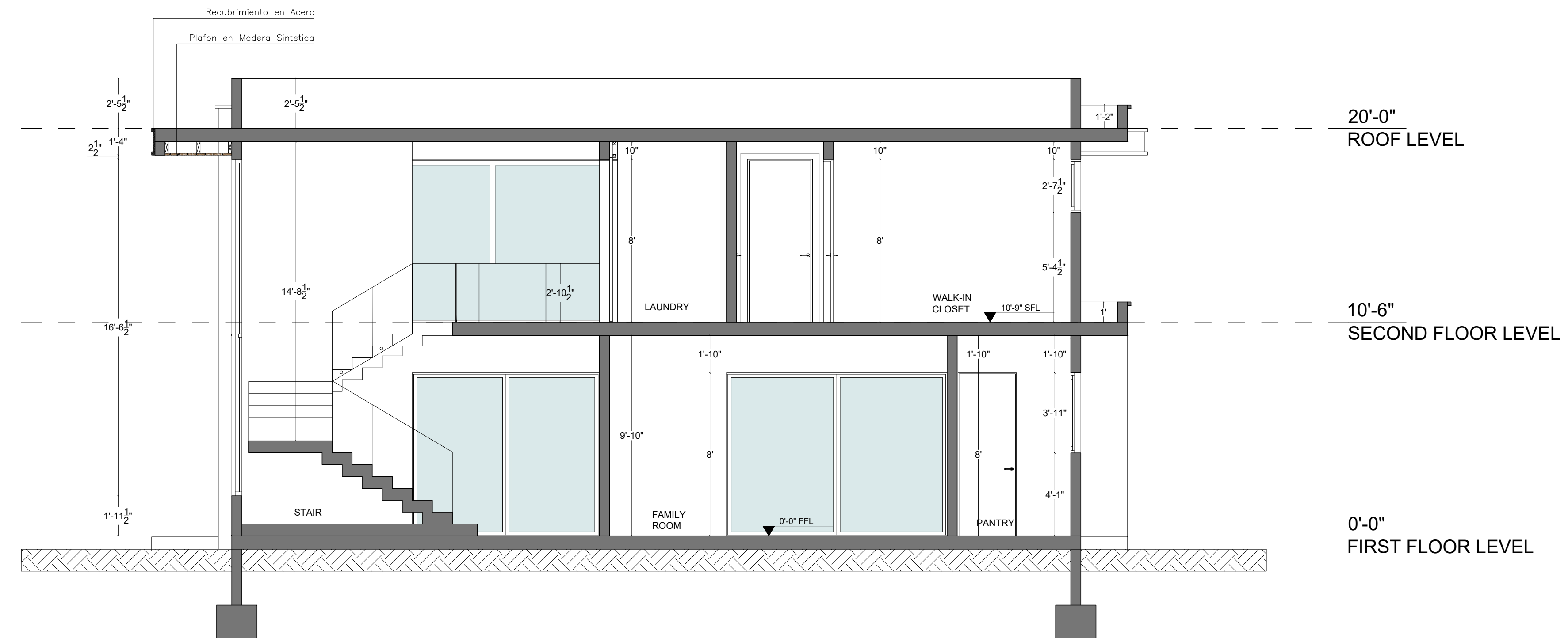
01 SECTION C - C
